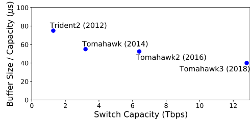
Figure 1: Hardware trends for top-of-the-line data center switches from Broadcom. Switch capacity and link speed have been growing rapidly, but buffer size is not keeping up with increases in switch capacity.
