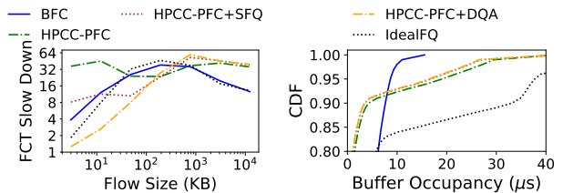
(a) FCT SlowDown (b) Buffer Occupancy
