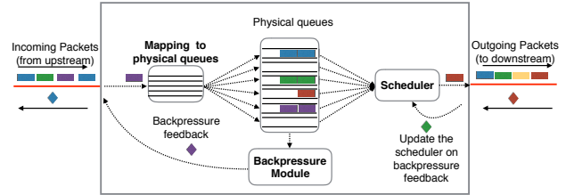
Figure 5: Logical switch components in per-hop, per-flow flow control.
