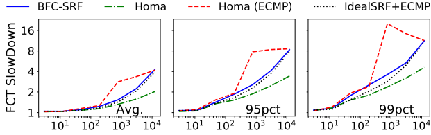
(b) Facebook Hadoop, 60%
