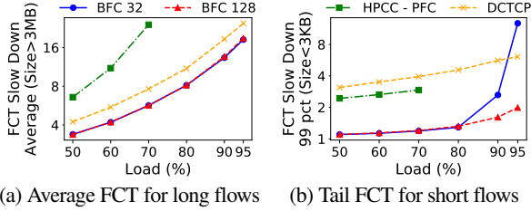
(a) Average FCT for long flows (b) Tail FCT for short flows Figure 12: Average FCT slowdown for long flows, and 99 th percentile tail FCT slowdown for small flows, as a function of load.
