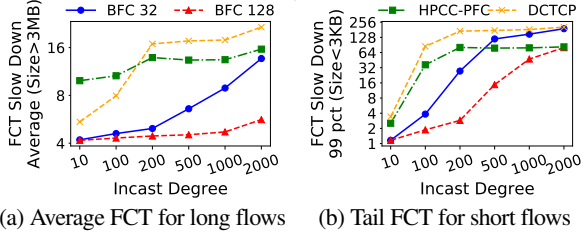
(a) Average FCT for long flows (b) Tail FCT for short flows Figure 13: Average FCT slowdown for long flows, and 99 th percentile tail FCT slowdown for small flows, as a function of incast degree.
