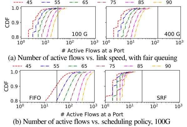
Figure 4: Number of active flows for different load, link speed, and scheduling policy. Lines correspond to different loads. Flow sizes are from the Google distribution with lognormal ( \sigma = 2 ) inter-arrival times.
