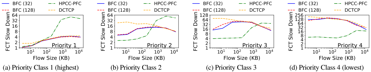
Figure 20: Multiple traffic classes with BFC, reporting 99 th percentile FCT slowdown for the Facebook workload, 60% load, and no incast.
