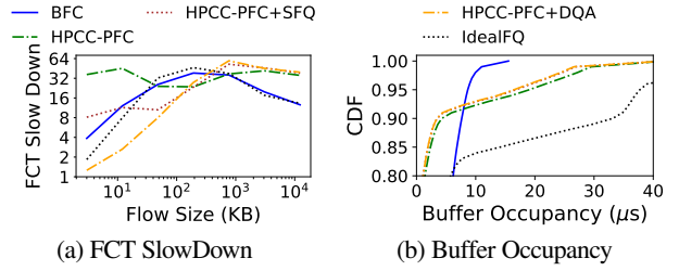
(a) FCT SlowDown (b) Buffer Occupancy Figure 14: FCT slowdown (99 th percentile) and buffer occupancy of HPCC variants, using the setup in Fig. 11a.
