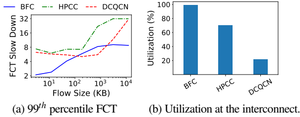
Figure 26: Performance in cross data center environment where two data center are connected by a 200 \mu s link, for the Facebook workload (60% load) with no incast traffic. The left figure shows the 99th percentile FCT slowdown for intra-data-center flows. The right figure shows the average utilization of the link connecting the two data centers.
