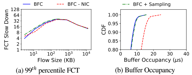
Figure 25: FCT slowdown (99 th percentile) and buffer occupancy distribution for two BFC variants. When NICs don't respond to backpressure (BFC - NIC), BFC experiences moderate increased buffering. Using sampling to reduce recirculation (BFC + sampling) has marginal impact on performance.
